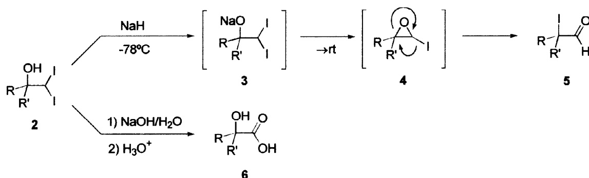
Scheme 1: Synthesis of \alpha -iodoaldehydes and \alpha -hydroxyacids
